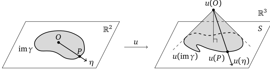
FIGURE 1. The point u(O) cannot be in the plane S and the curve \gamma is star-shaped.
