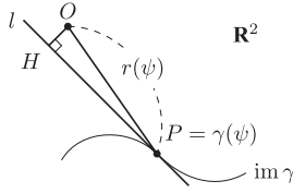
FIGURE 2. The function r is Lipschitz continuous.
