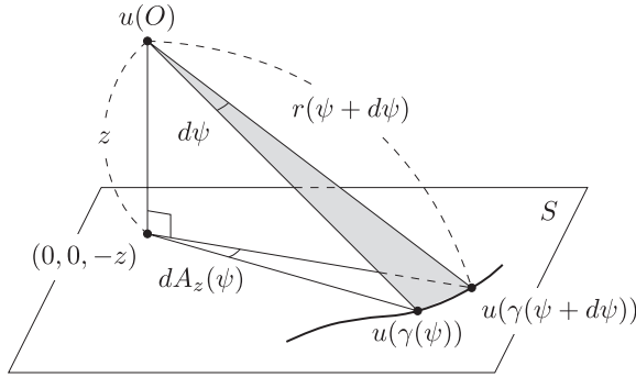
FIGURE 3. The infinitesimal triangle and its projection to the plane.
